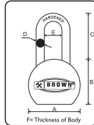
Shackle & Lock Body Dimensions (mm)
